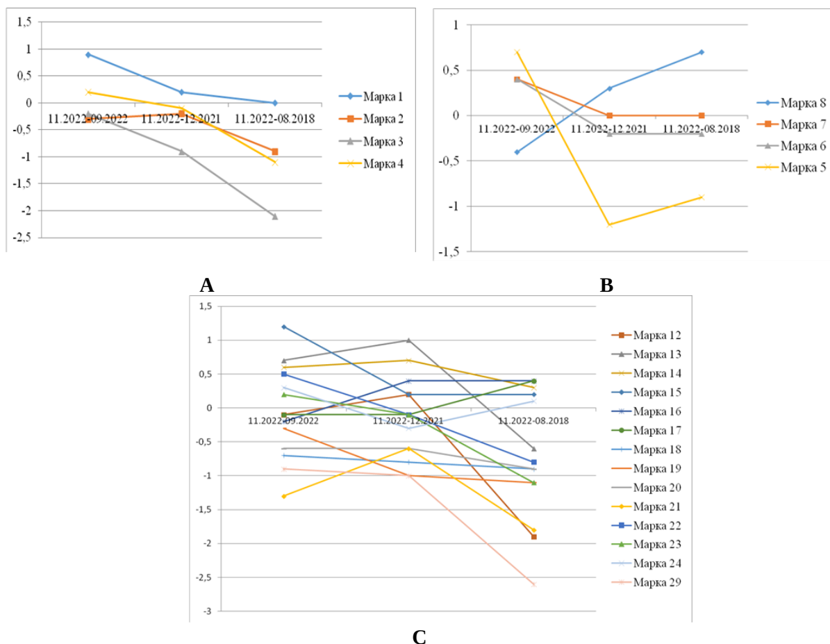
Figure 3. Dynamics of vertical movements of control marks between observation cycles: a - installed on the FWS building; b - installed on the BED building; c - installed on the TB building (source: developed by the author)
